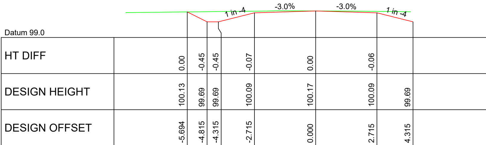
CHAINAGE 41.792
